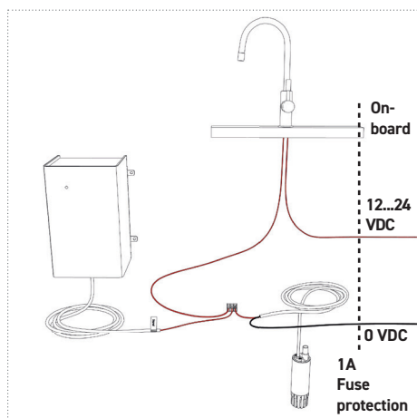
Figure 16: Electrical connection (signal) with submersible pump
