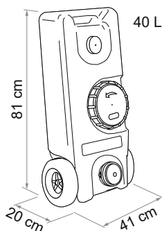
Roll-Tank 40 F
