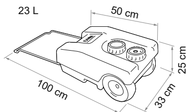
Roll-Tank 23 F
